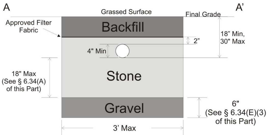
Trench Cross Section View
