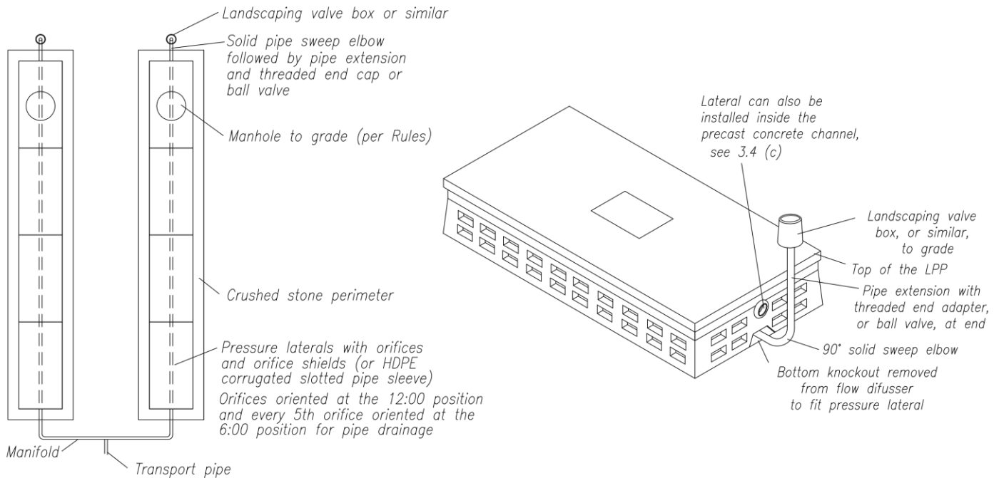
6.85 Figure 27: LPP Details for Shallow Concrete Chambers (Top and Isometric Views)
