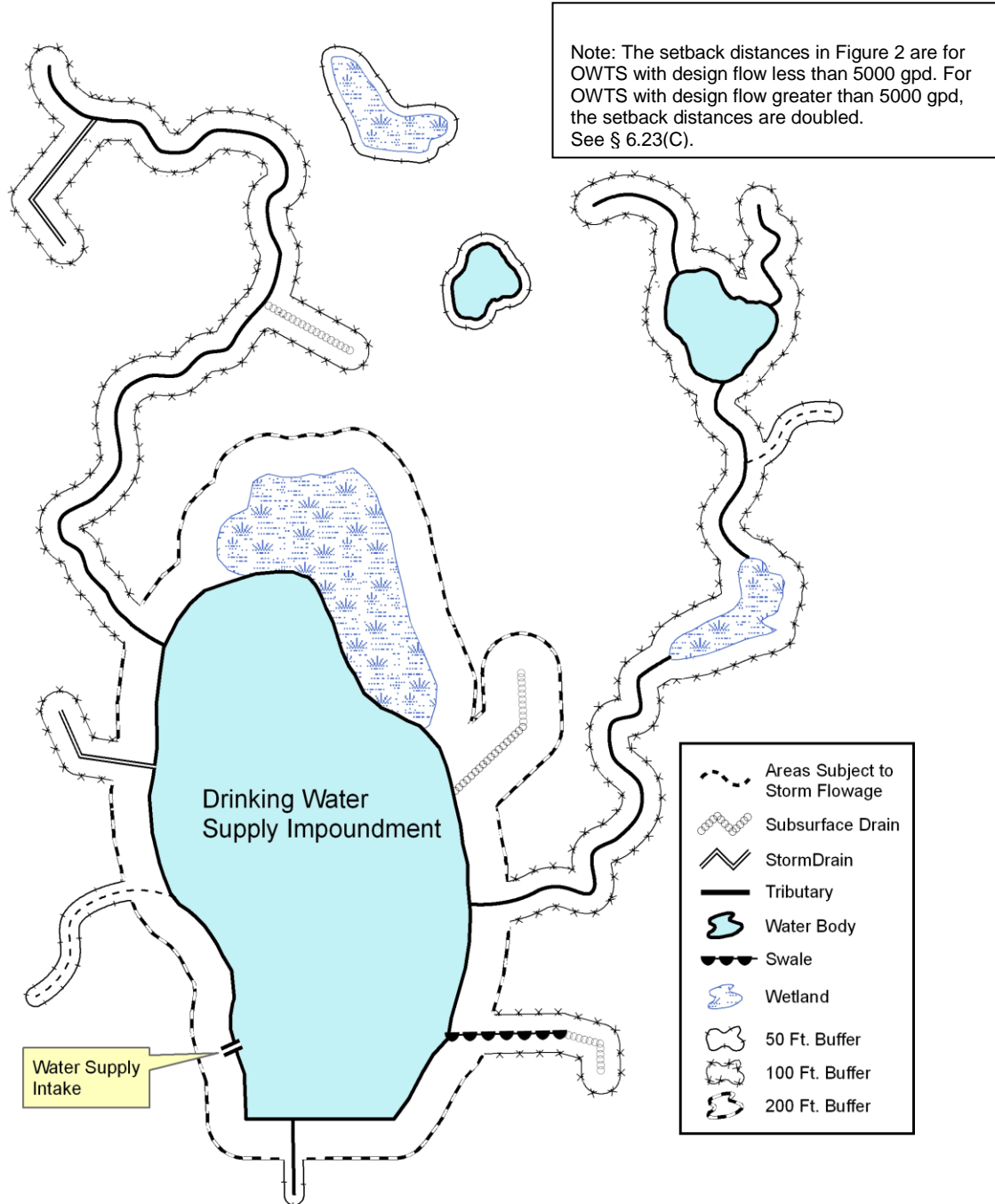
Figure 2 Minimum Setback Distances in Drinking Water Supply Watershed
